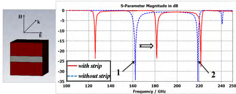
Fig. 1: a) A single dielectric cube with a metal strip b) The transmission coefficient S_{21} spectrum for the single dielectric cube with the metal strip
