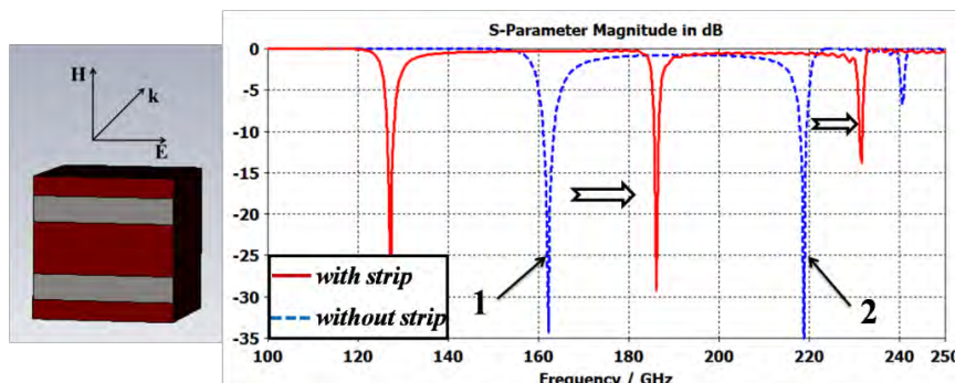
Fig. 4: a) A single dielectric cube with two metal strips b) The transmission coefficient S_{21} spectrum for the single dielectric cube with two metal strips.
